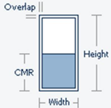
Double Hung Storm Window
